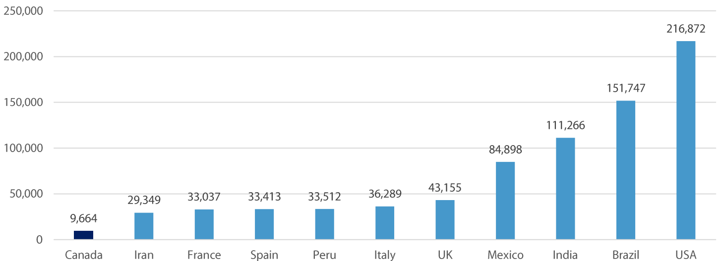
Cumulative Deaths (Top 10 plus Canada)
