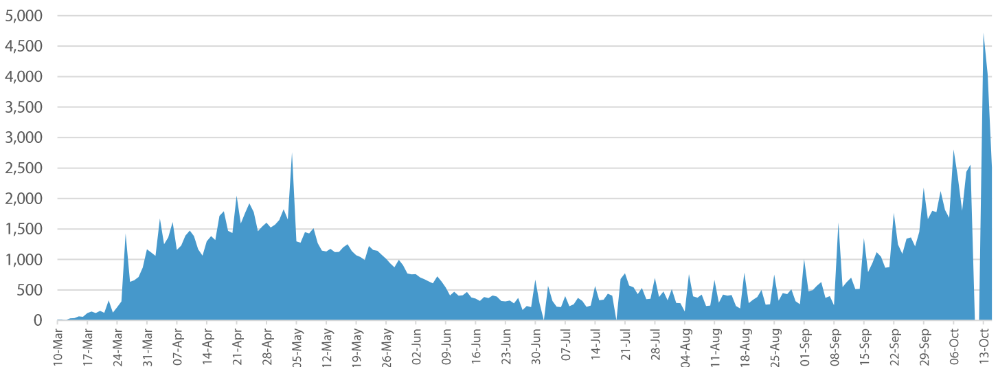
Canadian COVID-19 Cases by Date
