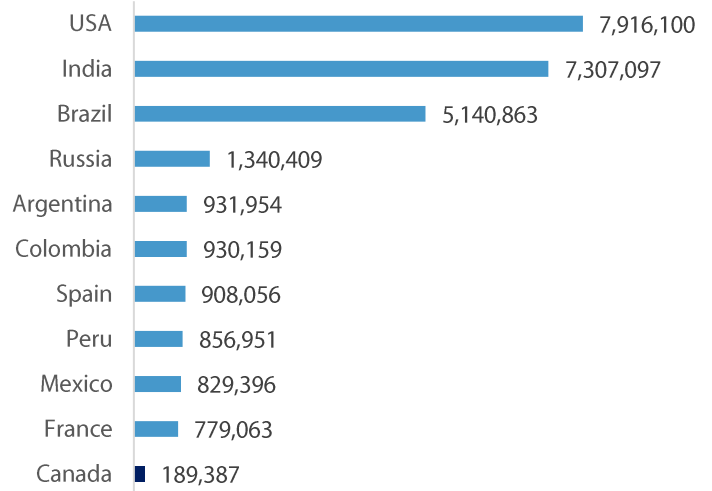
Cumulative Cases (Top 10 plus Canada)
